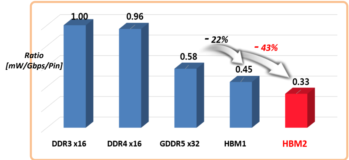
Power Efficiency @ IDD4R
